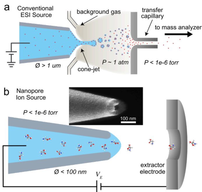
Figure 1: Comparison between a) conventional electrospray emission (ESI) ion beam source and b) the newly proposed nanopore ion source, which vaporizes charged molecules via ion field emission (IFE) 4
