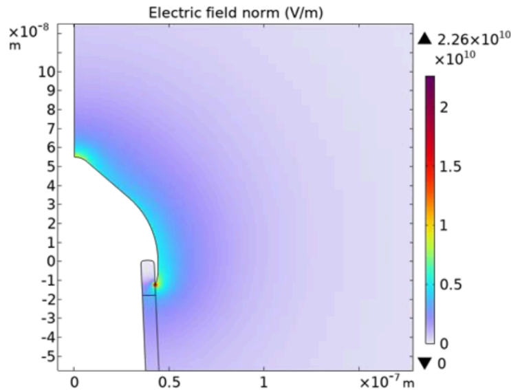
Figure 2: A simulation result of the electric field strength around the meniscus of the ion solution generated by a nanopore nozzle with an applied potential, courtesy of the Stein group at Brown
